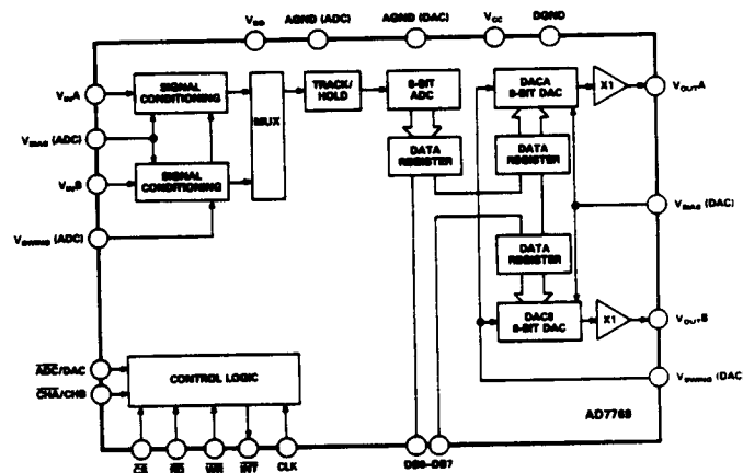
Figure 3. AD7769 Functional Block Diagram
