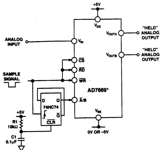
Figure 6. Infinite Sample-and-Hold Using AD7669
